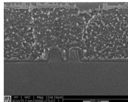
Figure 3 Picture showing the EO polymer filling the waveguide slot, an essential requirement to make the modulator work.
