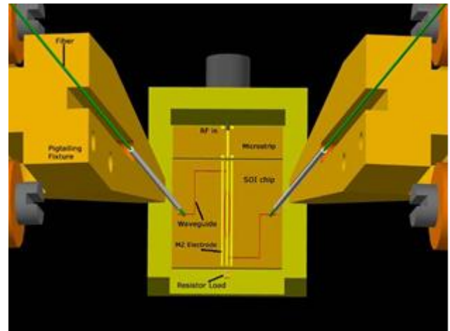
Figure 4 Fiber to grating couplers alignment procedure
