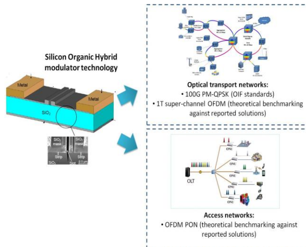
Figure 1 Specification definition structure of SOH modulator technology for long and short reach optical networks.
